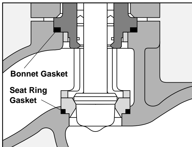
Figure 9: Body Gaskets
