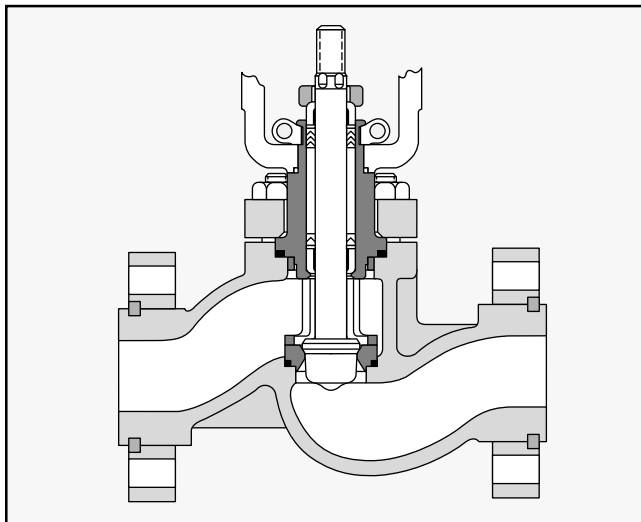
Figure 3: Globe-style Body
