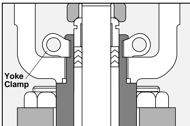
Figure 10: Yoke Clamp
