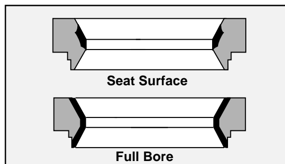
Figure 19: Hard Facing Variations – Seat
