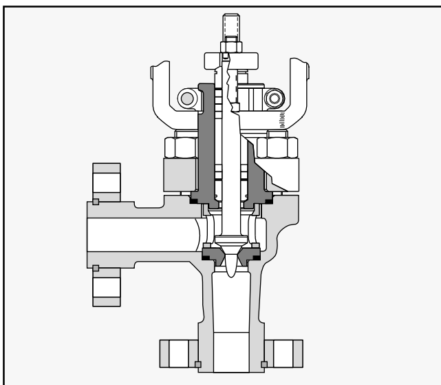
Figure 5: Angle-style Body
