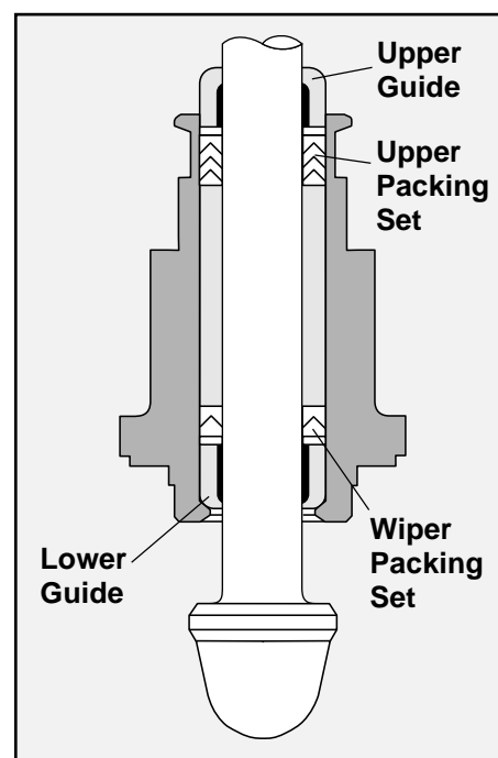
Figure 12: Typical PTFE V-ring Arrangement
