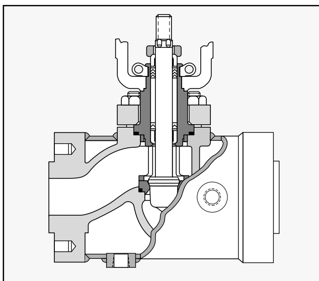
Figure 6: Steam-jacketed Body
