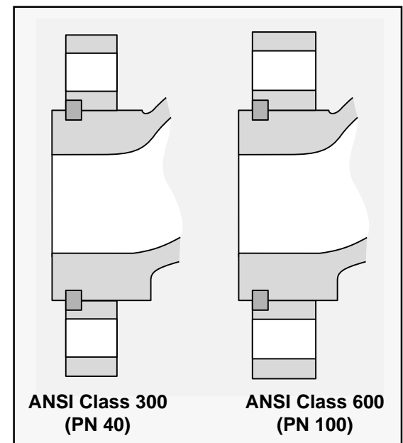
Figure 8: End Flanges
