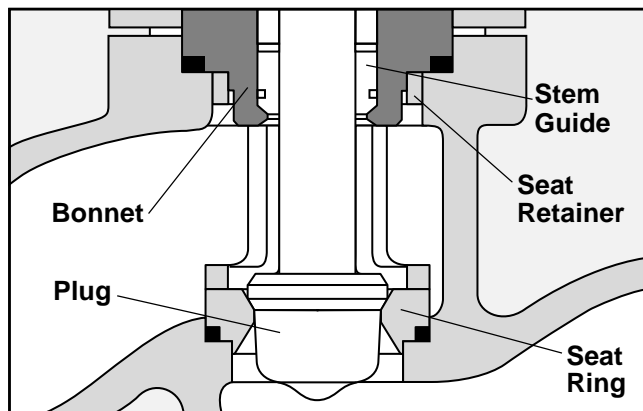
Figure 15: Standard Trim
