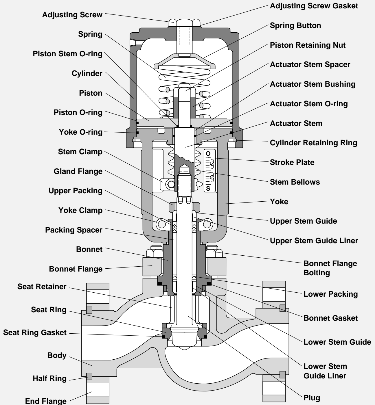
Figure 2: Mark One Control Valve
