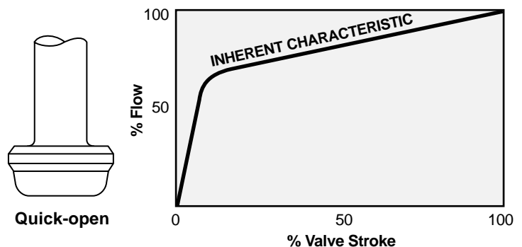
Figure 13: Flow Characteristics
