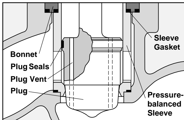
Figure 16: Pressure-balanced Trim
