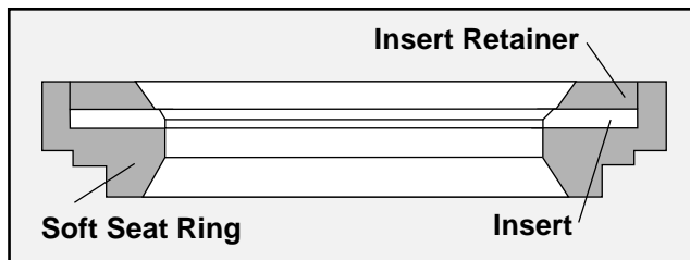
Figure 17: Typical Soft Seat Configuration
